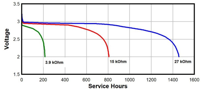
Various Continuous Discharge
