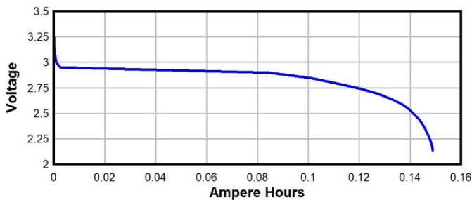
Rated Capacity test 15 kOhm Continuous to 2.0V
